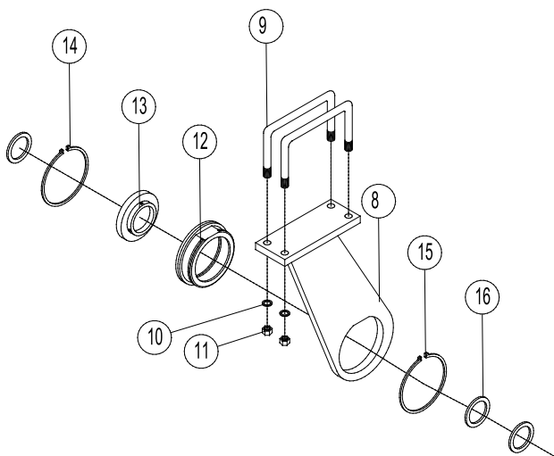
Support bearing for 8,2 m Vip-Roller NG wing section
